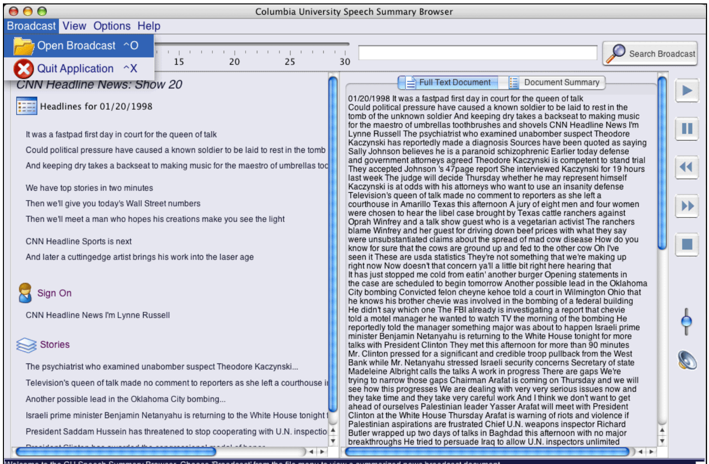
Figure 1. The user chooses to load a broadcast from the application menu. The speech browser allows a user to load an mp3 file of a CNN News broadcast that is accompanied by a BBN transcript.
